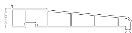
180mm A type cill AC 180
